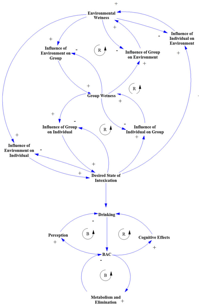
Figure 2 Causal loop diagram for drinking event system. [Colour figure can be viewed at wileyonlinelibrary.com ]
