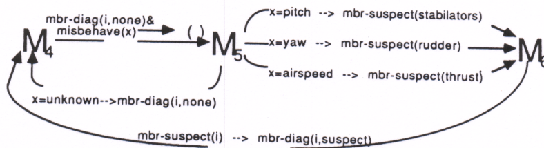
Fig. 8. KR graph of model based reasoning.
